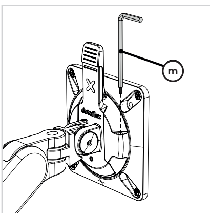
anti-theft / anti-diefstal Anti-Diebstahl / anti-vol antirrobo / antifurto
